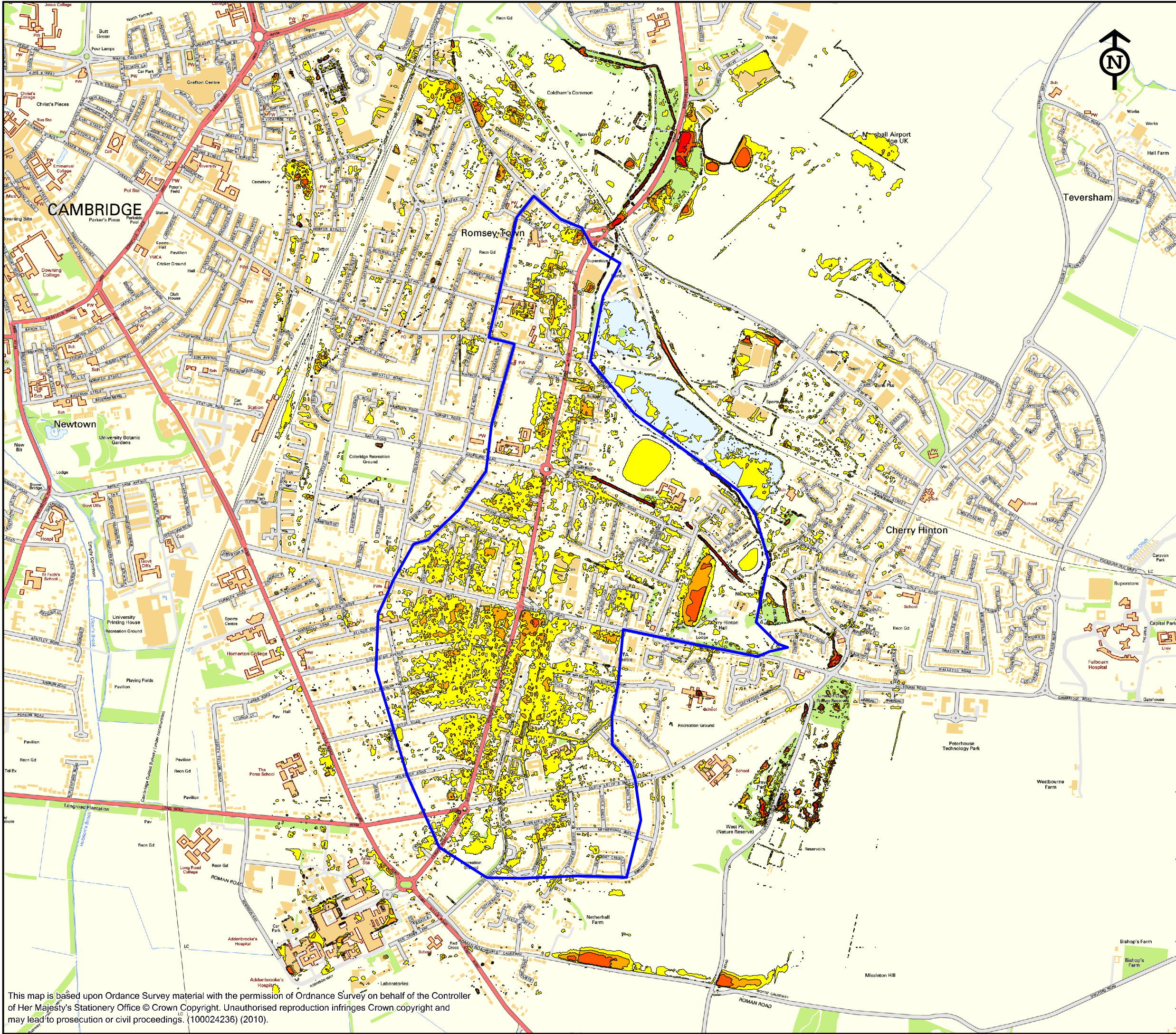
FIGURE G34 0.5% AEP "OPTION C6" PLUVIAL MODELLING MAXIMUM DEPTH CHERRY HINTON
